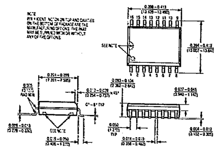
S Package 16-Lead Plastic SOL
